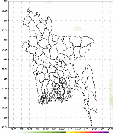
Accumulated Rainfall (mm) Period (22-01-2025 to 01-02-2025)
