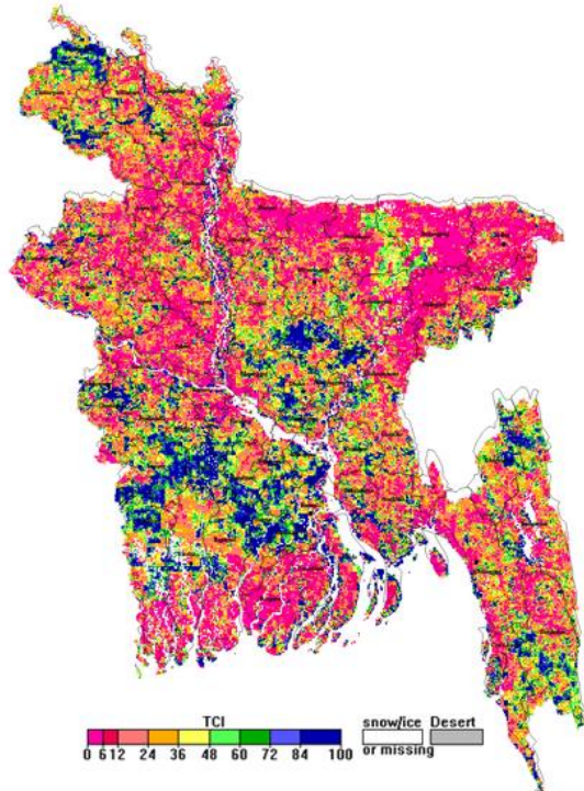
NOAA/ AVHRR BLENDED TCI composite for the week No. 25 (18 June-24 June) over Agricultural regions of Bangladesh
