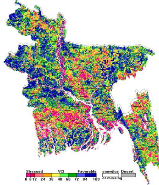
NOAA/ AVHRR BLENDED VCI composite for the week No. 25 (18 June-24 June) over Agricultural regions of Bangladesh
