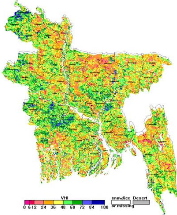
NOAA/ AVHRR BLENDED VHI composite for the week No. 25 (18 June-24 June) over Agricultural regions of Bangladesh
