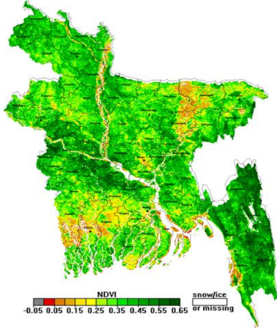
NOAA/VIIRS BLENDED NDVI composite for the week. No. 25 (18 June-24 June) over Agricultural regions of Bangladesh
