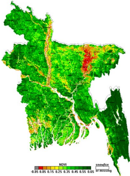
NOAA/VIIRS BLENDED NDVI composite for the week. No. 35 (27August- 02 September) over Agricultural regions of Bangladesh
