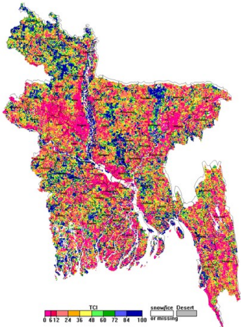
NOAA/ AVHRR BLENDED TCI composite for the week No. 35 (27August- 02 September) over Agricultural regions of Bangladesh
