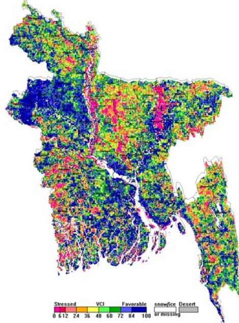
NOAA/ AVHRR BLENDED VCI composite for the week No. 35 (27August- 02 September) over Agricultural regions of Bangladesh
