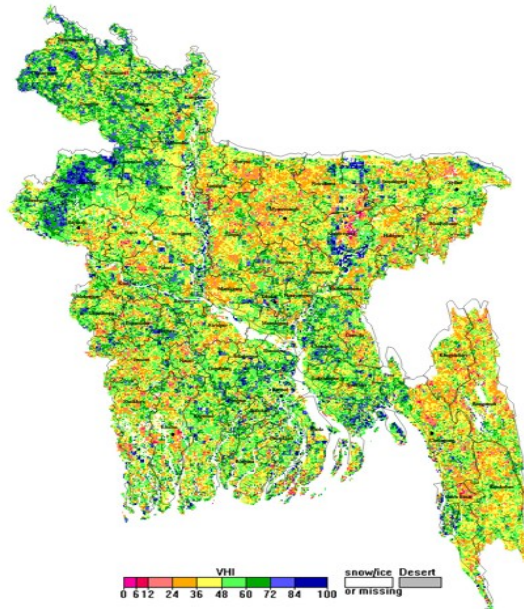
NOAA/ AVHRR BLENDED VHI composite for the week No. 35 (27August- 02 September) over Agricultural regions of Bangladesh
