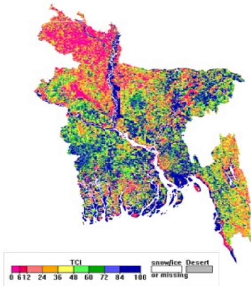
NOAA/ AVHRR BLENDED TCI composite for the week No. 44 (29 October-04 November) over Agricultural regions of Bangladesh
