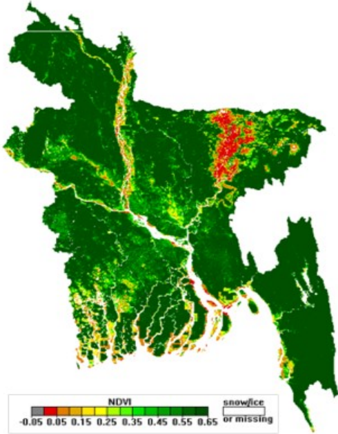
NOAA/VIIRS BLENDED NDVI composite for the week. No. 44 (29 October-04 November) over Agricultural regions of Bangladesh
