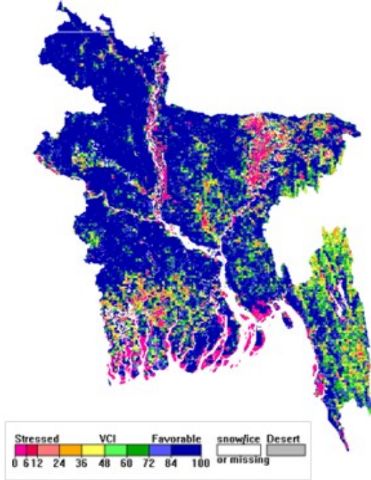
NOAA/ AVHRR BLENDED VCI composite for the week No. 44 (29 October-04 November) over Agricultural regions of Bangladesh
