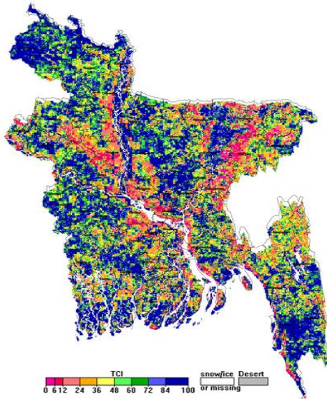
NOAA/ AVHRR BLENDED TCI composite for the week No. 38 (15 September -21 September) over Agricultural regions of Bangladesh
