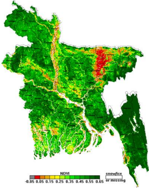
NOAA/VIIRS BLENDED NDVI composite for the week No. 38 (15 September -21 September) over Agricultural regions of Bangladesh
