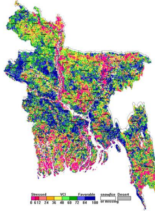
NOAA/ AVHRR BLENDED VCI composite for the week No. 38 (15 September -21 September) over Agricultural regions of Bangladesh
