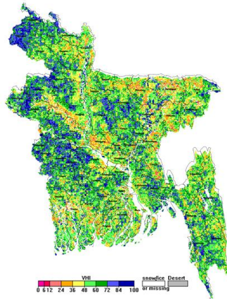
NOAA/ AVHRR BLENDED VHI composite for the week No. 38 (15 September -21 September) over Agricultural regions of Bangladesh
