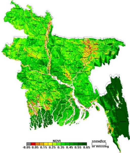
NOAA/VIIRS BLENDED NDVI composite for the week. No. 02 (08 January-14 January) over Agricultural regions of Bangladesh
