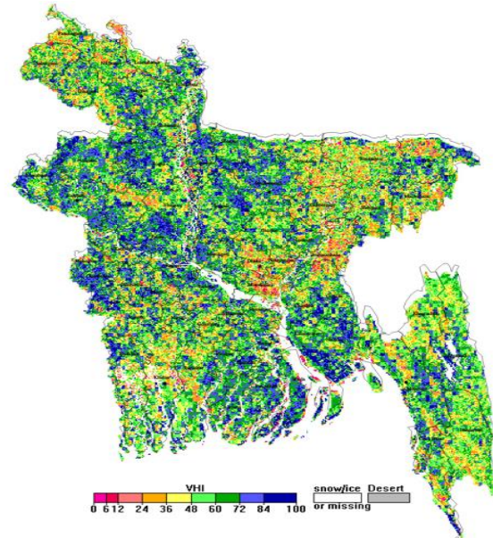
NOAA/ AVHRR BLENDED VHI composite for the week 02 (08 January-14 January) over Agricultural regions of Bangladesh
