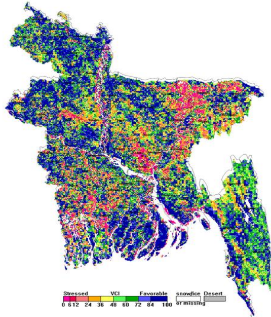
NOAA/ AVHRR BLENDED VCI composite for the week No. 02 (08 January-14 January) over Agricultural regions of Bangladesh
