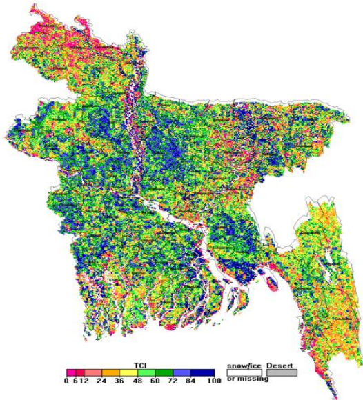
NOAA/ AVHRR BLENDED TCI composite for the week 02 (08 January-14 January) over Agricultural regions of Bangladesh
