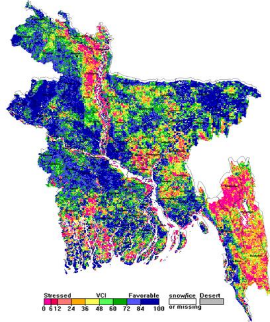
NOAA/ AVHRR BLENDED VCI composite for the week No. 19 (07 May-13 May) over Agricultural regions of Bangladesh
