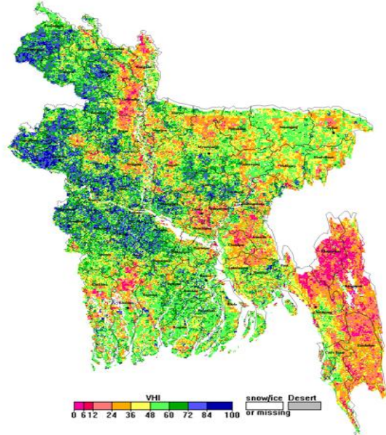
NOAA/ AVHRR BLENDED VHI composite for the week No. 20 (14 May-20 May) over Agricultural regions of Bangladesh
