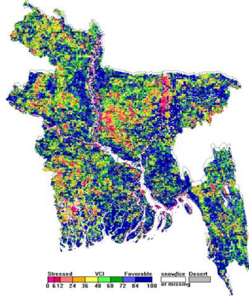
NOAA/ AVHRR BLENDED VCI composite for the week No. 28 (09July- 15July) over Agricultural regions of Bangladesh
