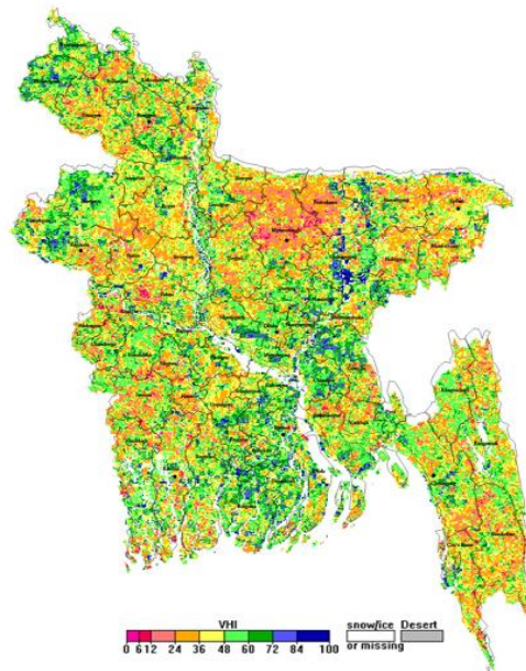
NOAA/ AVHRR BLENDED VHI composite for the week No. 32 (06 August- 12 August) over Agricultural regions of Bangladesh
