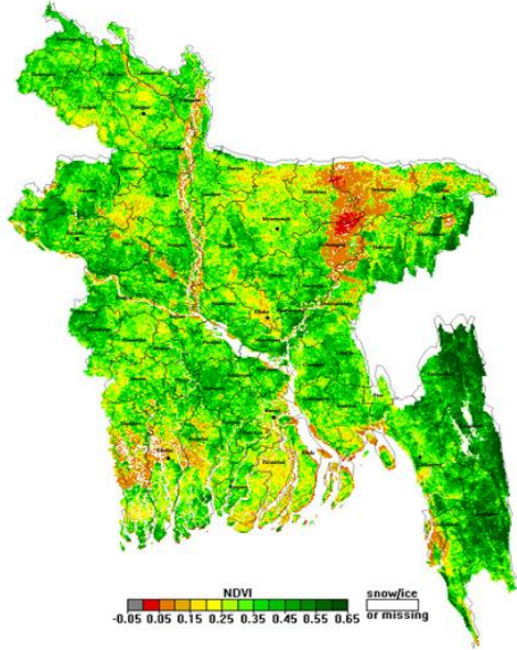
NOAA/VIIRS BLENDED NDVI composite for the week No. 32 (06 August- 12 August) over Agricultural regions of Bangladesh
