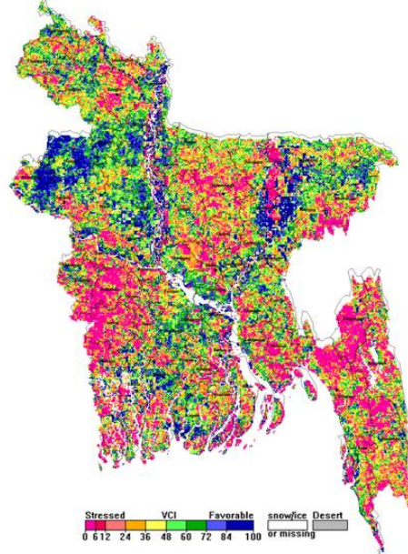
NOAA/ AVHRR BLENDED VCI composite for the week No. 32 (06 August- 12 August) over Agricultural regions of Bangladesh
