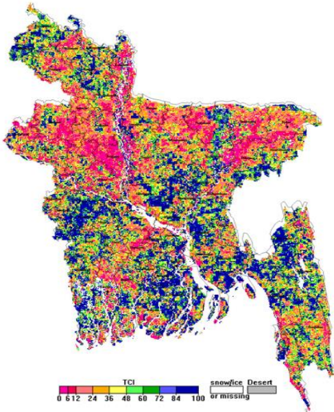
NOAA/ AVHRR BLENDED TCI composite for the week No. 32 (06 August- 12 August) over Agricultural regions of Bangladesh
