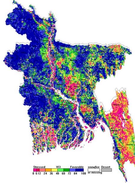
NOAA/ AVHRR BLENDED VCI composite for the week No. 17 (23 April-29 April) over Agricultural regions of Bangladesh
