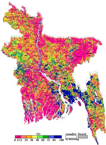
NOAA/ AVHRR BLENDED TCI composite for the week No. 22 (21 May-27 May) over Agricultural regions of Bangladesh
