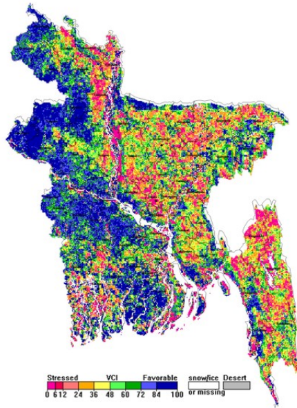
NOAA/ AVHRR BLENDED VCI composite for the week No. 22 (21 May-27 May) over Agricultural regions of Bangladesh
