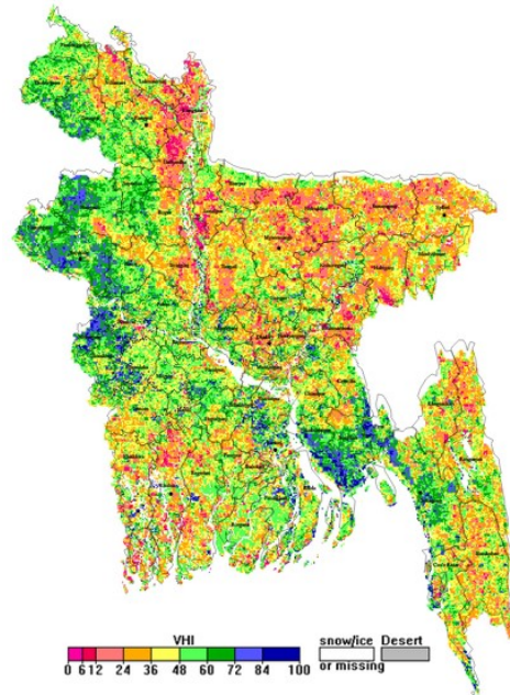
NOAA/ AVHRR BLENDED VHI composite for the week No. 22 (21 May-27 May) over Agricultural regions of Bangladesh
