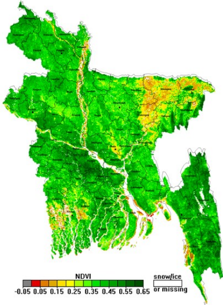
NOAA/VIIRS BLENDED NDVI composite for the week. No. 22 (21 May-27 May) over Agricultural regions of Bangladesh
